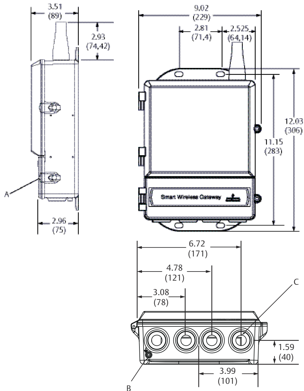
Figure 1: Wireless Gateway
