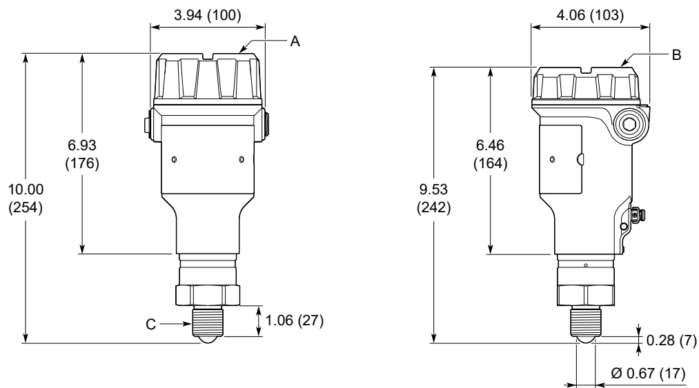
Figure 13: Lens Antenna with 3/4-in. Threaded Process Connection
