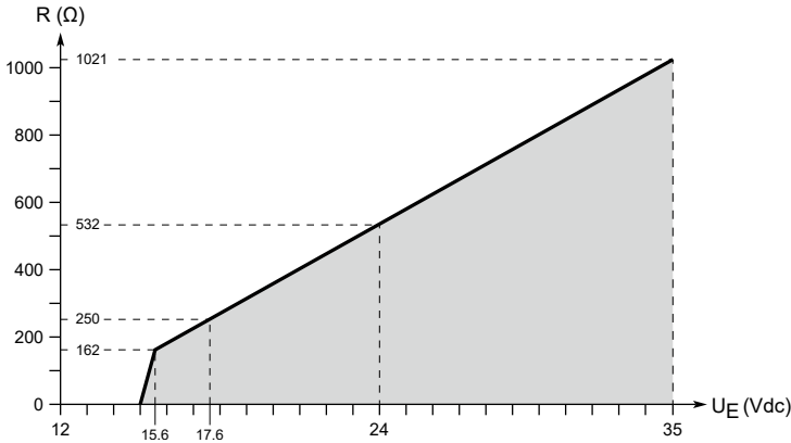
Figure 4: Load Limits
