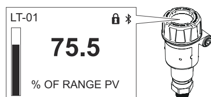
Figure 5: LCD Display
