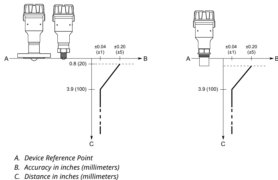
Figure 3: Accuracy Over Measuring Range
